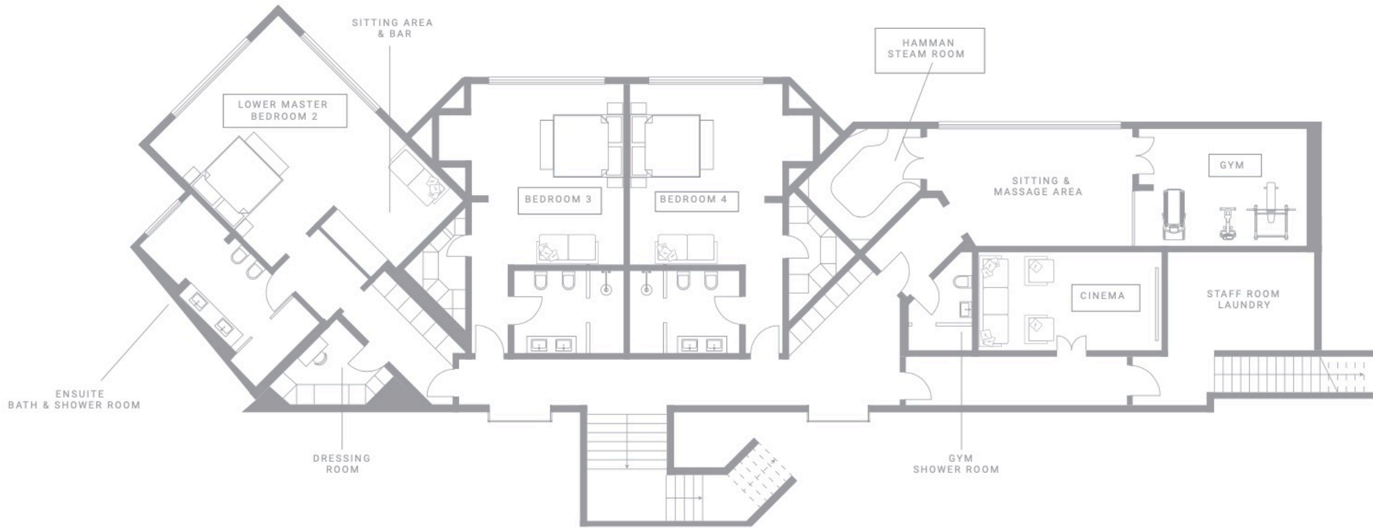
MAIN HOUSE GROUND FLOOR
